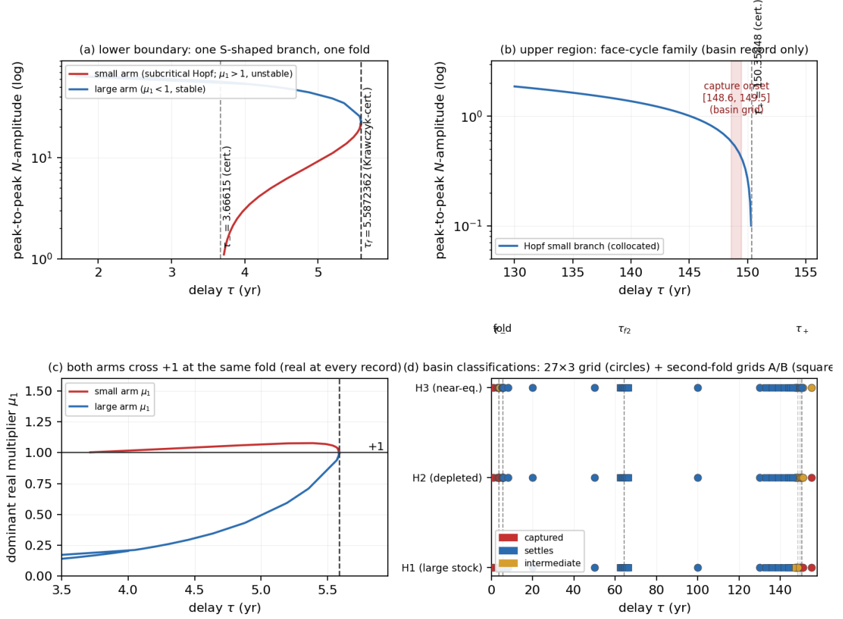
Figure 1: The five-regime attractor topology from the two pre-registered continuation records (five-regime campaign and second-fold campaign; every panel drawn from the deposited campaign CSVs, see Data availability). (a) The lower S-branch: the subcritical-Hopf small arm (red, \mu_1 > 1 ) and the stable large arm (blue, \mu_1 < 1 ) meet at the single Krawczyk-certified fold \tau_f = 5.5872362 yr. (b) The upper S-branch: the unstable arm from the Hopf at \tau_+ folds at the certified \tau_{f2} = 64.4023272 yr and returns as a stable arm (inset: its real multiplier through the fold), with the basin capture onset [148.6, 149.5] yr — a basin boundary, not a fold — and the certified \tau_+ = 150.35848 yr. (c) The lower branch's dominant real multipliers crossing +1 at the same fold. (d) Basin classifications (captured / settles / intermediate) on both registered grids ( 27 \times 3 plus the second-fold grids A/B, dt = 0.02 ): the depleted history is captured at \tau = 5.575 ; every tested history settles from 5.6 to 146 (H1 intermediate at 145–146); capture returns only inside [148.6, 149.5] yr.
